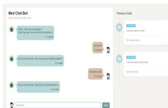
Fig4: Result Prediction
