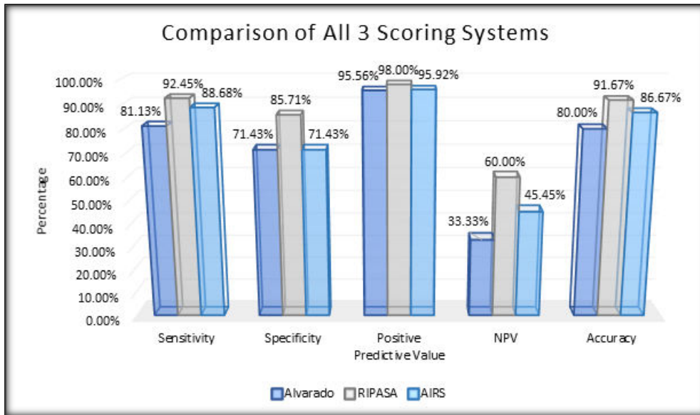
Figure 1: Comparison of Alvarado, RIPASA, and AIRS Scoring Systems
