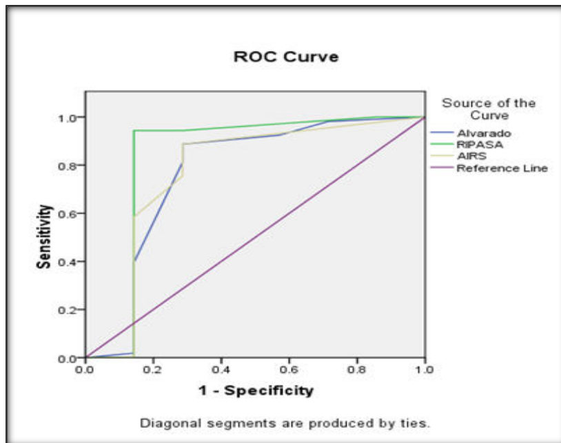
Figure 2: Receiver Operator Characteristic Curve
