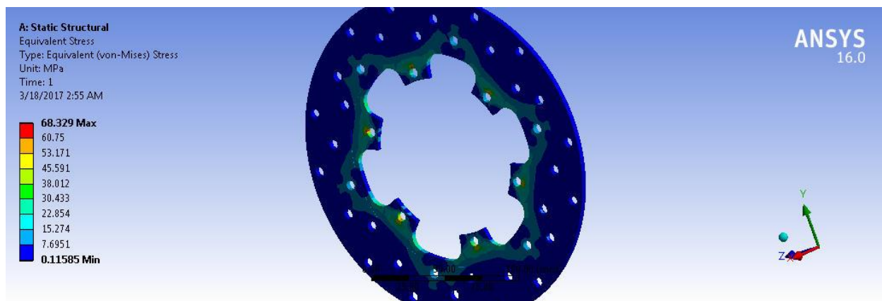
Figure 6 Equivalent Stress of Disc Brake
