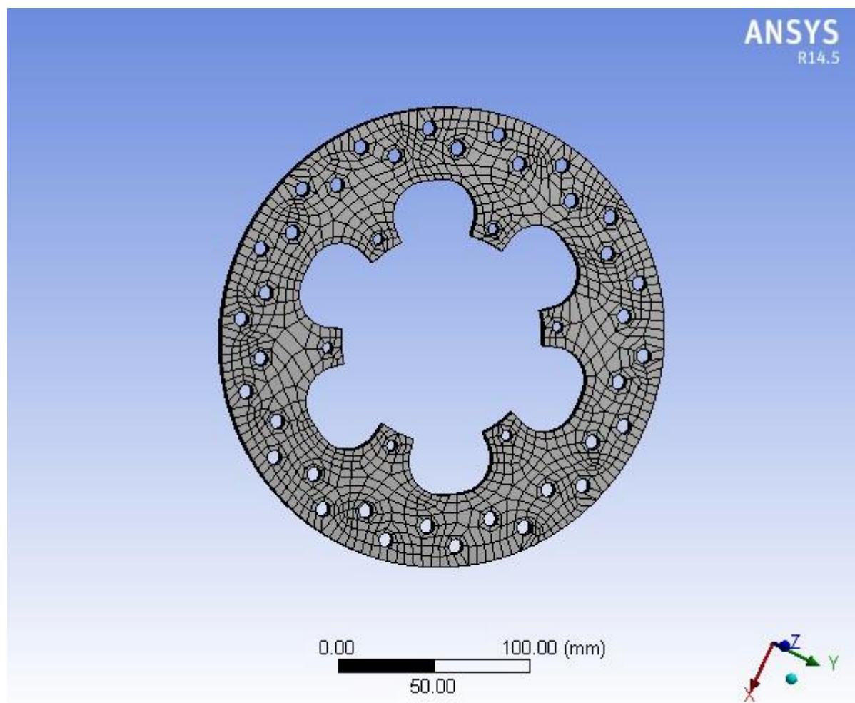
Figure 2 Meshed Model of the Disc brake
