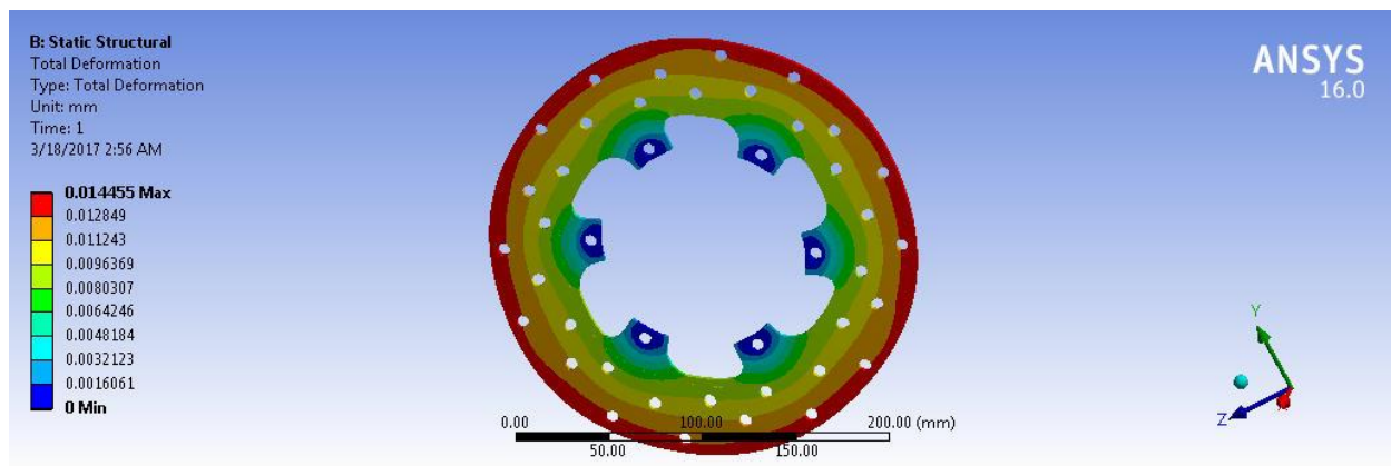
Figure 4 Total Deformation of Disc Brake
