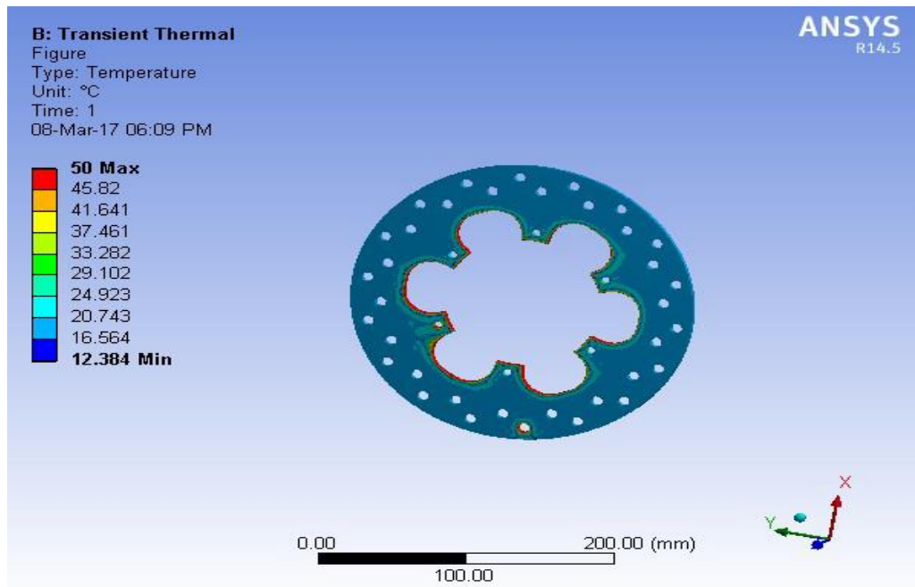
Figure 7 Temperature Distribution of Disc Brake
