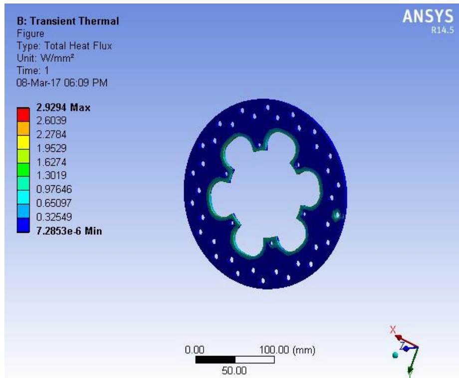
Figure 8 Total Heat Flux of Disc Brake
