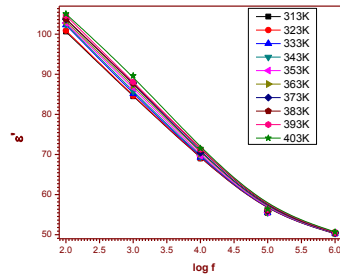
Figure 4. Variation of \epsilon' with \log f for LHP Crystal
