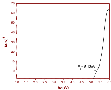
Figure 3. Tauc's Plot of LHP Crystal
