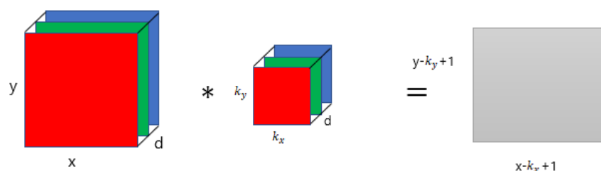
Fig. 3: Representation of convolution layer process.
