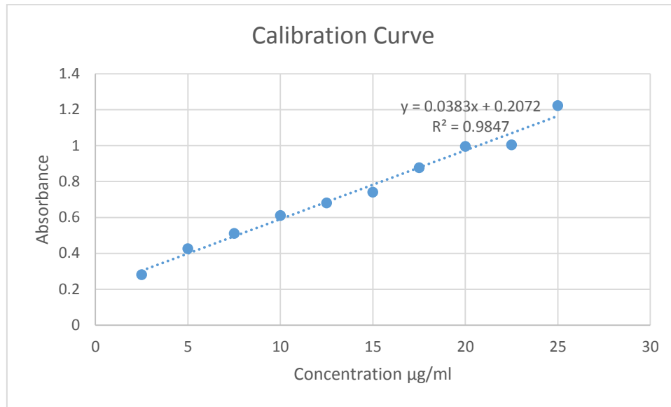
Figure 4: Calibration Curve
