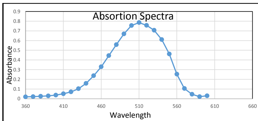
Figure 3: Absorption spectra showing \lambda_{\text{max}} 510nm
