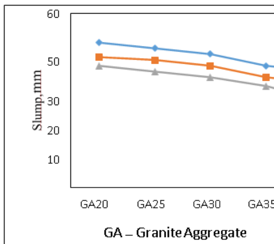
Fig.4.1. Slump of RAC 20
