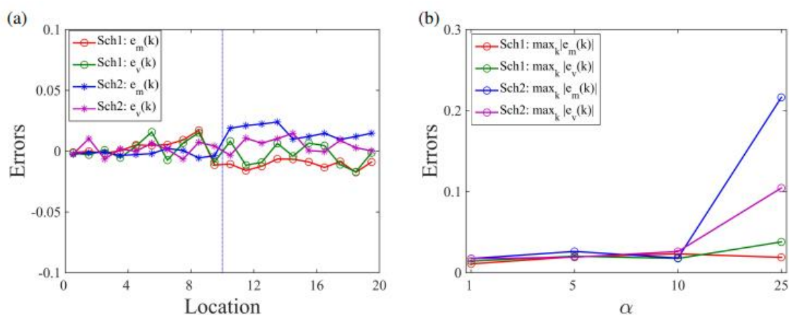
Fig. 5 (a) The mean number of morphogens in C2 at time t = 50 s. Different simulation methods are compared with \alpha = 10, 20, 30, 40, 50 (with a static boundary): the Gillespie SSA with multigrid discretization ( \alpha grid points with size \Delta x and one grid point with size h ), Scheme 1, Scheme 2, and Scheme 2 with no noise due to diffusion in \Omega_s . (b) The probability distribution of the normalized morphogen number in C1 with Scheme 2. The probability distributions are computed for X^{\ell}(t)/\Delta x, \ell = 1, 2, \dots, \alpha and compared among the cases with \alpha = 10, 50 (with a static boundary) at time t = 0.01, 50 s. Initially, 50 molecules are located in \Omega_s in panels (a) and (b).
