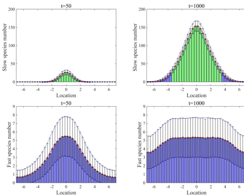
Fig. 8 Mean numbers of the molecules of slow-diffusing pom1p clusters and fast-diffusing pom1p particles, and their standard deviations from the means at t = 50, 1000 s computed
