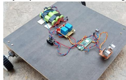
Figure 7: Hardware Kit of obstacle Avoiding Robot Car
