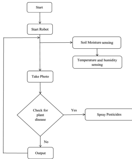
Figure 6: Program Flowchart
