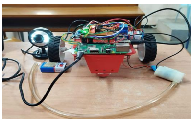
Figure 8: Project Module
