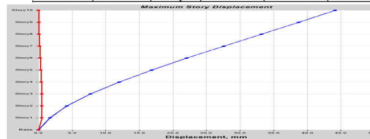
Figure 13: Storey displacements of structure with infill walls and without soft storey for EQ X using RSM
