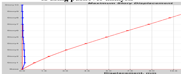
Figure 16: Storey displacements of structure with infill walls and without soft storey for Push Y using pushover analysis
