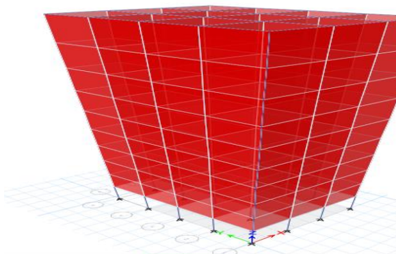
Figure 8: 3-D view of building with infills and with soft storey
