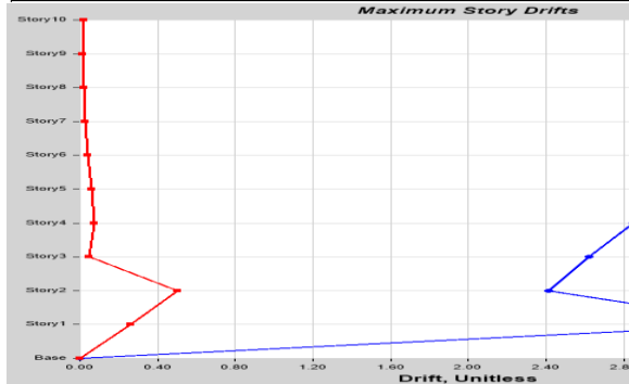
Figure 11: Storey drifts of structure with infill walls and soft storey for EQ X using RSM
