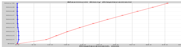
Figure 10: Storey displacements of structure with infill walls and soft storey for EQ Y using RSM
