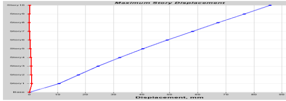
Figure 9: Storey displacements of structure with infill walls and soft storey for EQ X using RSM
