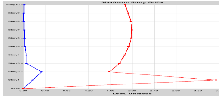
Figure 12: Storey drifts of structure with infill walls and soft storey for EQ Y using RSM Analysis Results of G+10 Building with Infill Walls and without Soft Storey Response Spectrum method
