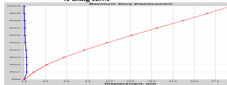
Figure 14: Storey displacements of structure with infill walls and without soft storey for EQ Y using RSM
