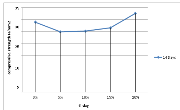
GRAPH 3.3.-SHOWING COMPRESSIVE STRENGTH FOR 14 DAYS
