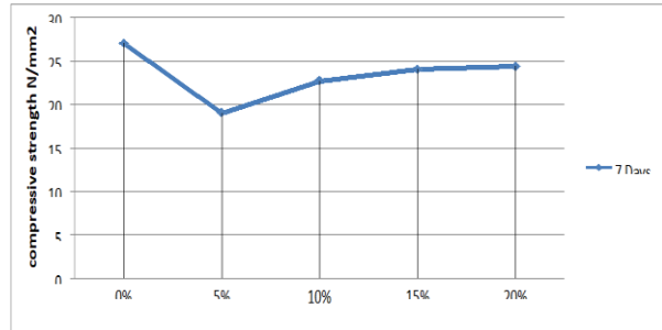
GRAPH 3.2- SHOWING COMPRESSIVE STRENGTH FOR 7 DAYS
