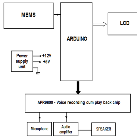
Figure 4: Proposed System Block Diagram
