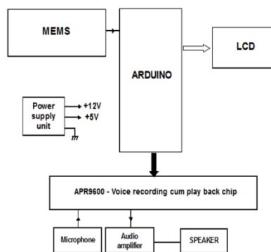
Fig 1.– Block diagram of Earthquake detector
