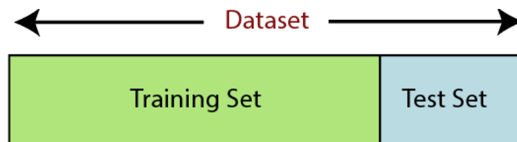
Fig. 2: Data splitting.
