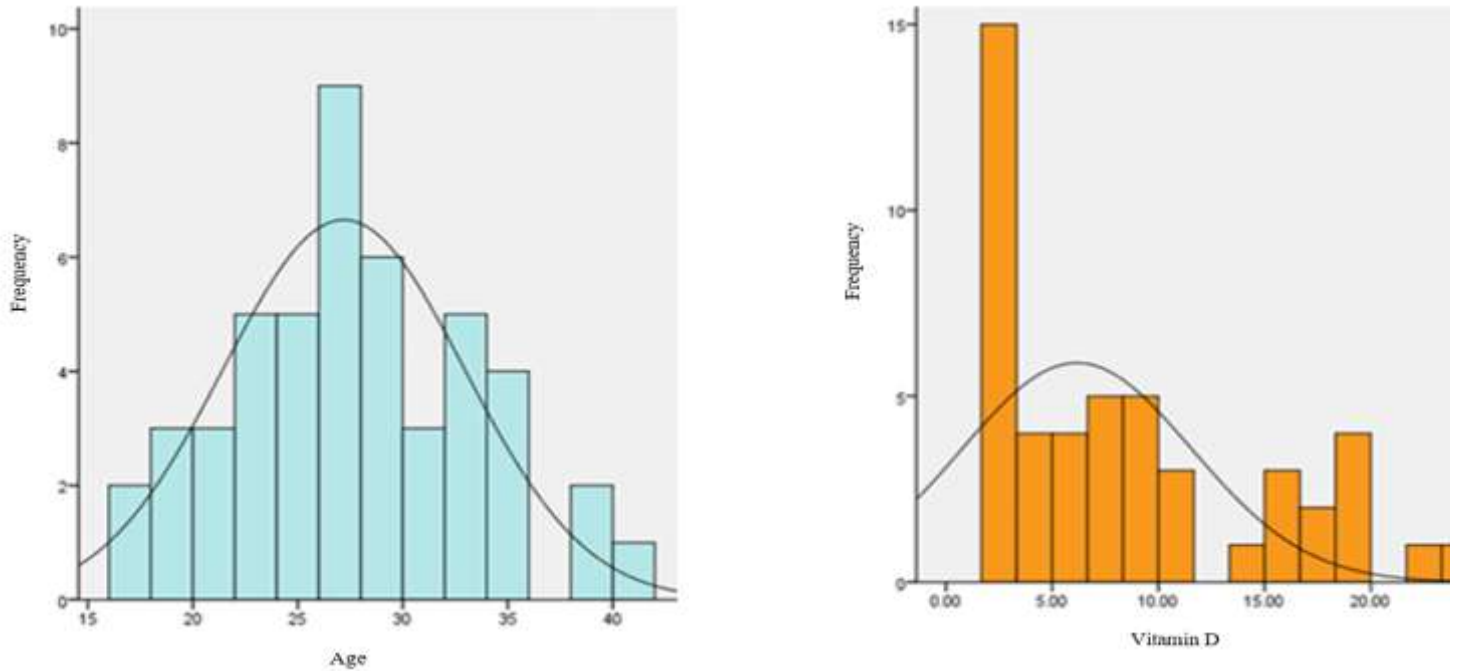
Figure 2: the distribution of age data and vitamin D levels in annual cold season samples
