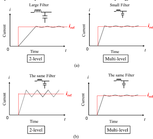
Fig. 3. Example of current waveforms in step response depending on the number of output levels and output filter of converters. (a) When both filters
