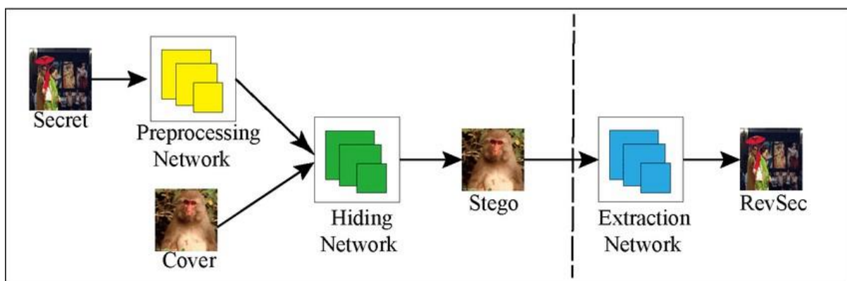
Fig. 1: Image steganography architecture.
