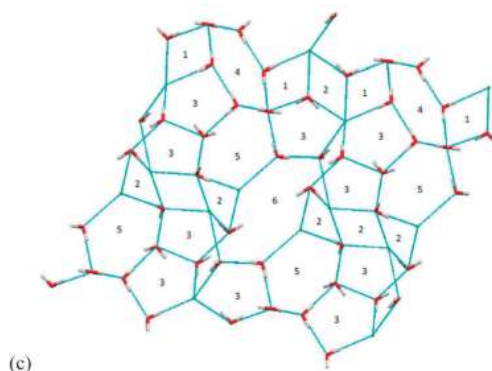
Fig. 2 (a) Ru(II) cationic building block 2 showing (arbitrary view) hydrogen bonding interactions between chloride anions and water molecules, (b) a closer view of the cyclic water–chloride cluster in 2, (c) nonplanar 2D anionic layer (arbitrary view) generated by the water–chloride cluster \{[(\text{H}_2\text{O})_{10}\text{Cl}_2] 2\}_n .
