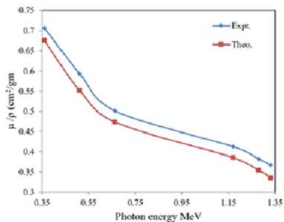
Fig. 2: Plots of photon energy versus mass attenuation coefficient of spinel ferrite composite \text{Ni}_{0.5}\text{Mn}_{1.5}\text{Cd}_{0.2}\text{Fe}_2\text{O}_4
