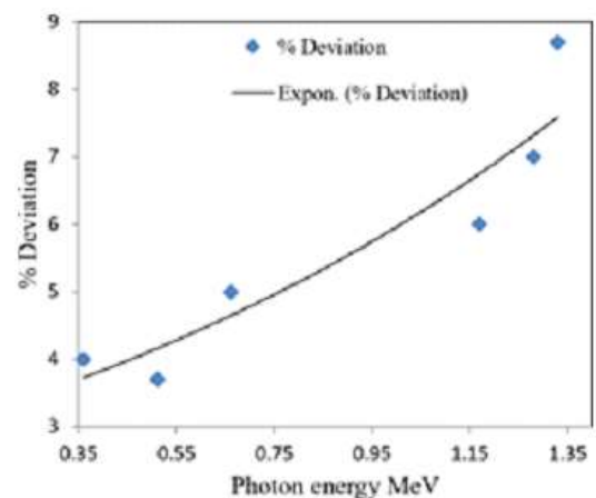
Fig.3: Plots of photon energy versus % deviation of theoretical and experimental values of mass attenuation coefficient of spinel ferrite composite \text{Ni}_{0.5}\text{Mn}_{1.5}\text{Cd}_{0.2}\text{Fe}_2\text{O}_4
