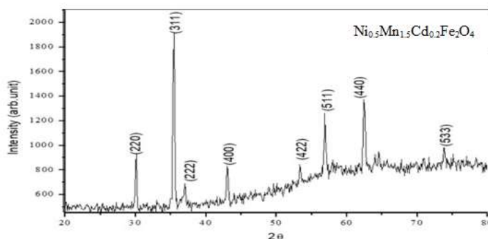
Fig. 1: X-ray diffraction patterns of spinel ferrite composite \text{Ni}_{0.5}\text{Mn}_{1.5}\text{Cd}_{0.2}\text{Fe}_2\text{O}_4 .
