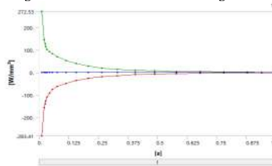
Graph 11: Result Directional Heat Flux of Triangular Fin
