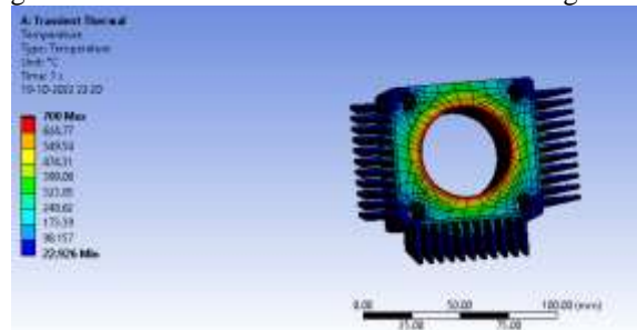
Fig 40: Transient Thermal Convection of Rectangular Fin
