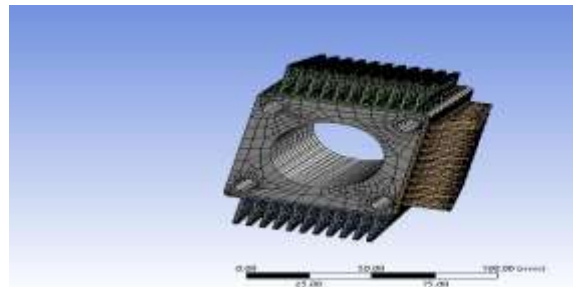
Fig 32: Mesh model
