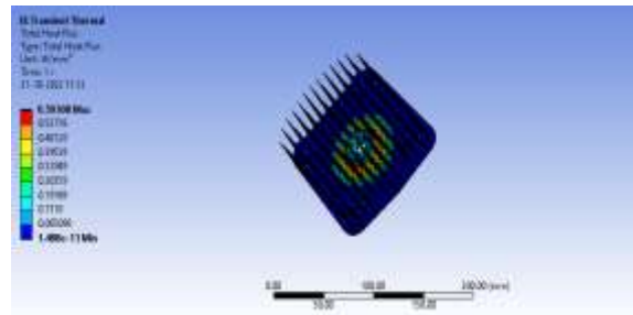
Fig 29: Total Heat Flux of Triangular Fin
