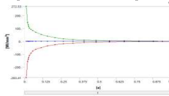
Fig 30 Directional Heat Flux of Triangular Fin
