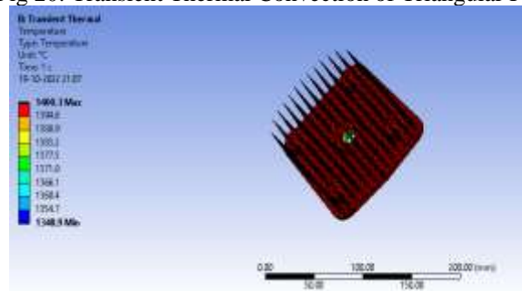
Fig 21: Temperature of Triangular Fin
