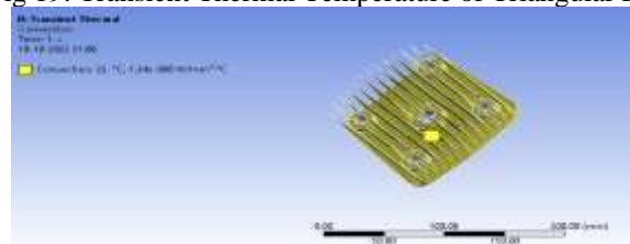
Fig 20: Transient Thermal Convection of Triangular Fin
