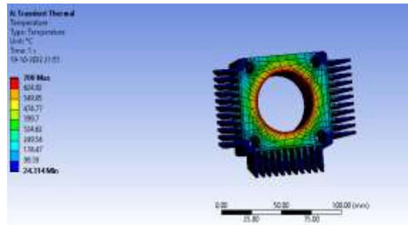
Fig 35: Temperature of Rectangular Fin
