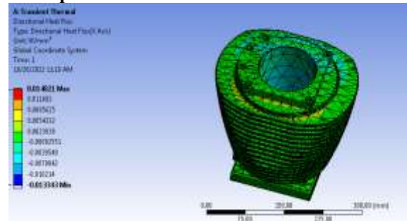
Fig 9: Directional Heat Flux of Circular Fin
