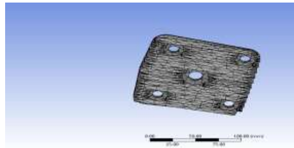
Fig 25: Triangular Mesh
