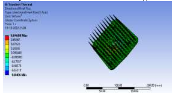
Fig 23: Directional Heat Flux of Triangular Fin
