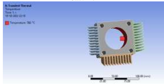
Fig 39: Transient Thermal Temperature of Rectangular Fin
