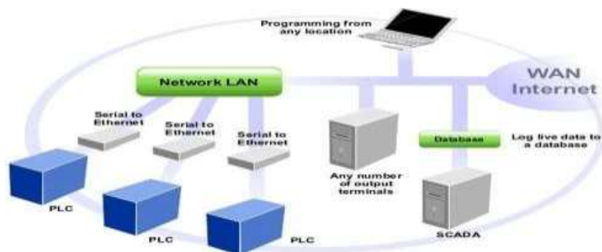
SCADA Architecture
