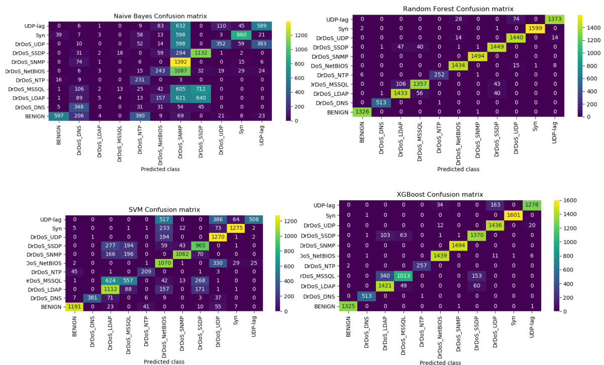
Fig. 4: Obtained confusion matrices for various machine learning algorithms.
