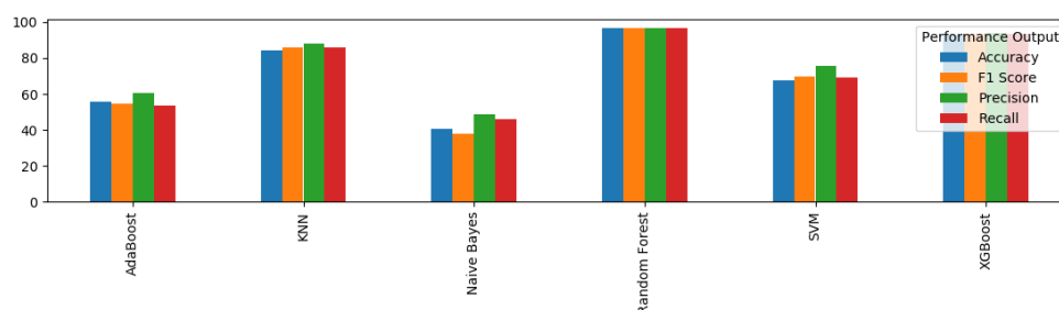
Fig. 5: Performance comparison of machine learning algorithms for DDoS attack detection.
