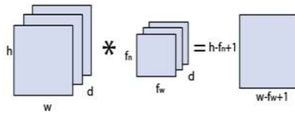
Fig 4. Convolution Layer structure
