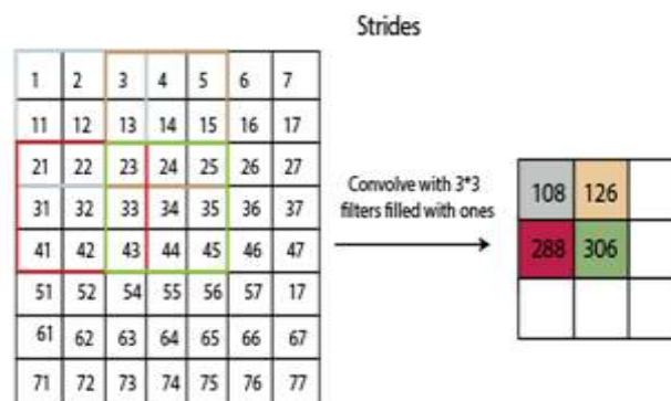
Fig 5. Stride's structure
