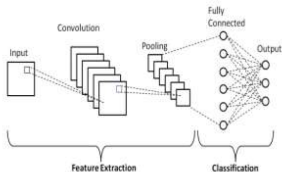
Fig 3.CNN Architecture
