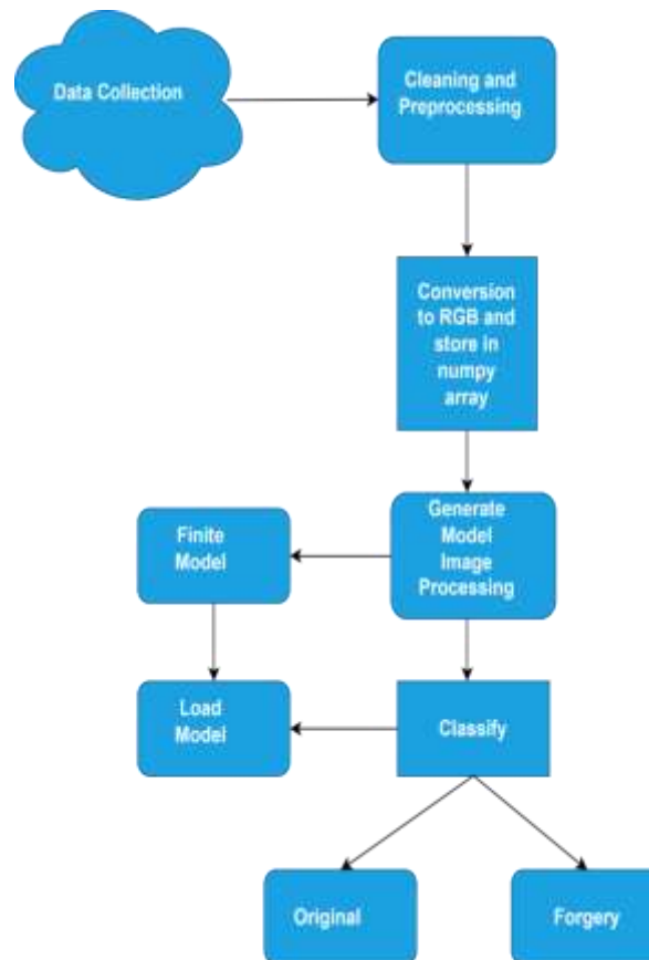
Fig 2. System Architecture
